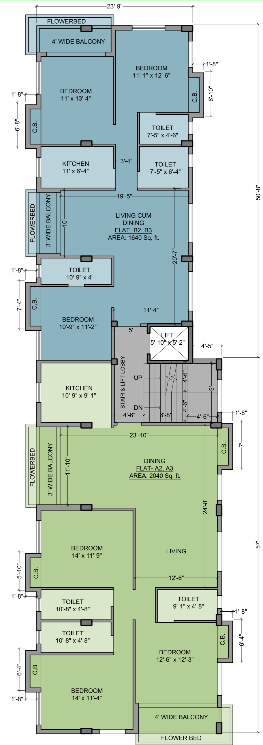
2nd.-3rd. FLOOR PLAN
