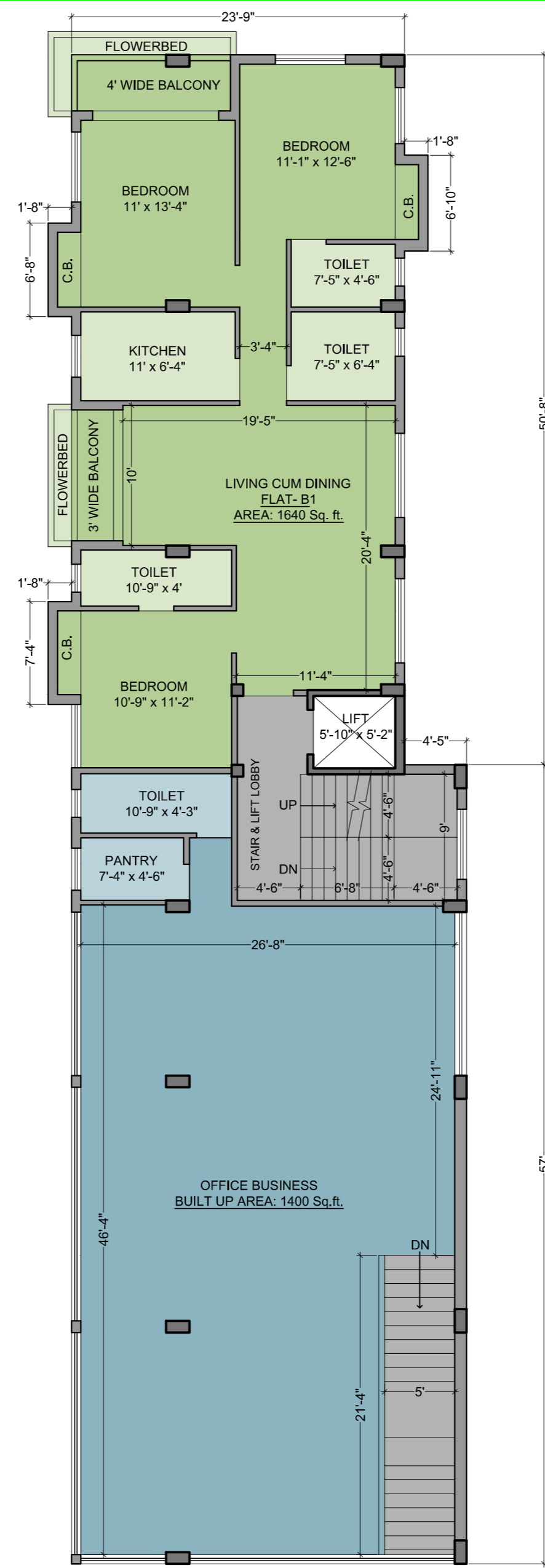
1st. FLOOR PLAN
